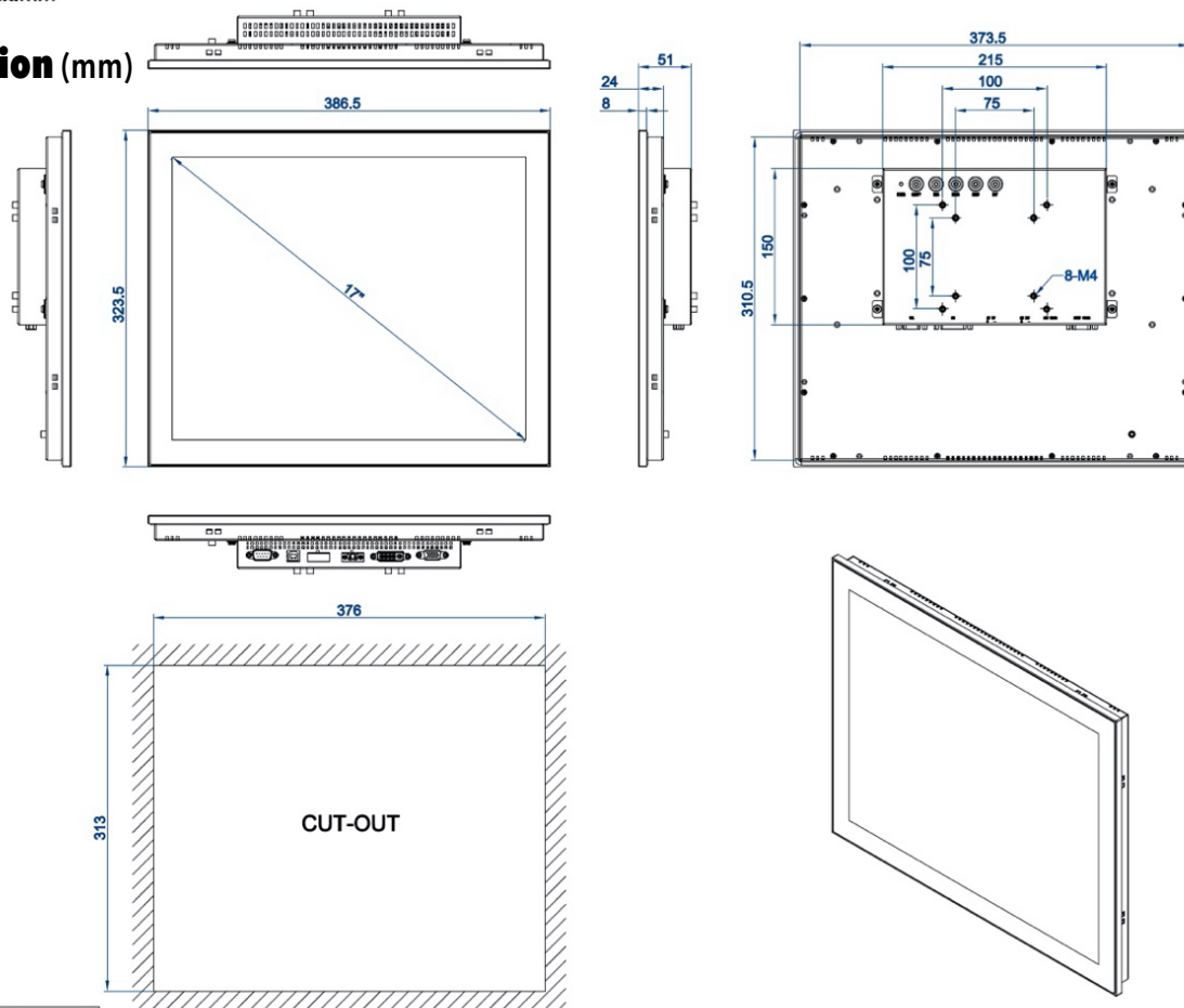
DIMENSIONAL DRAWING:TM-PC170
