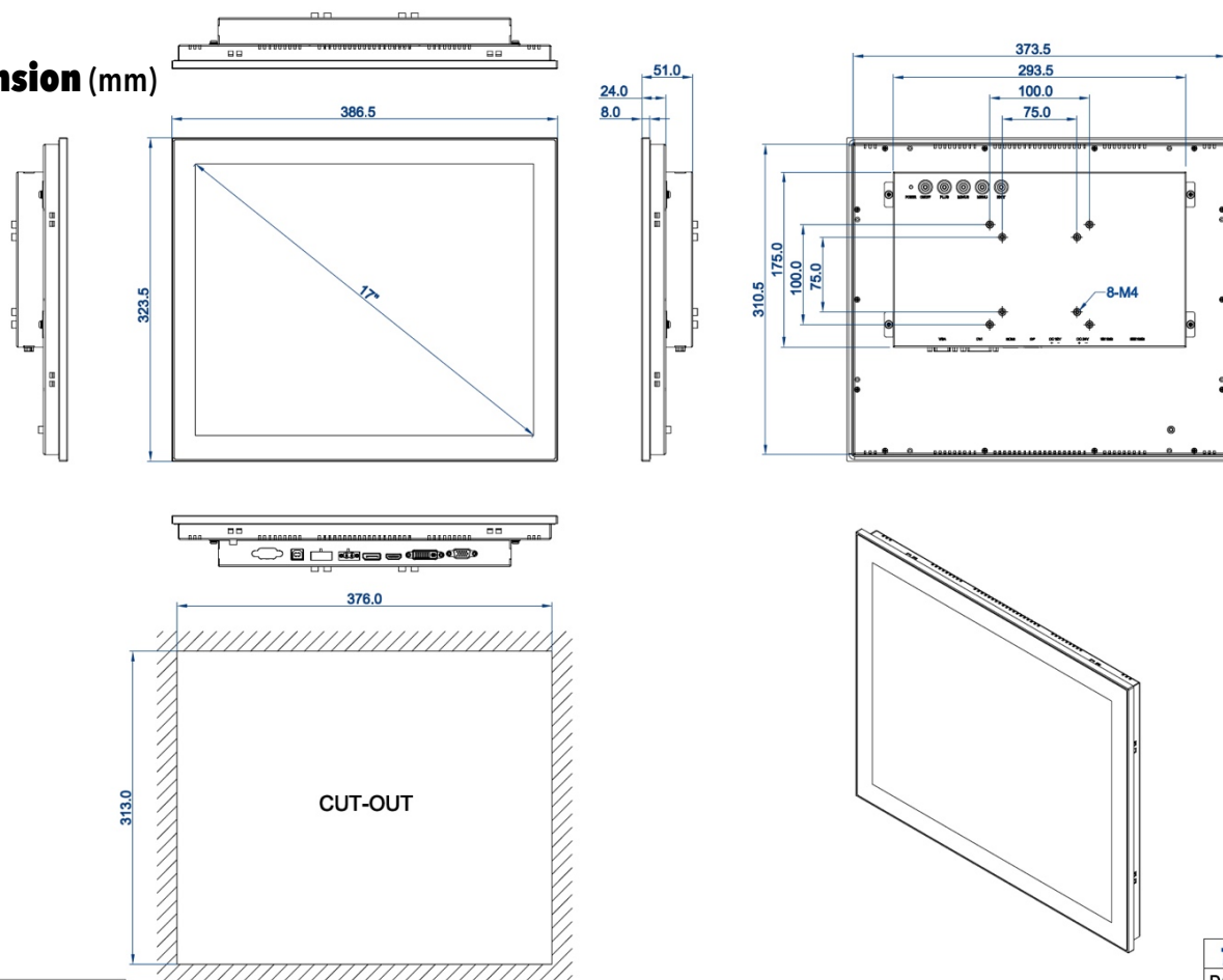
DIMENSIONAL DRAWING:TM-PCA170
