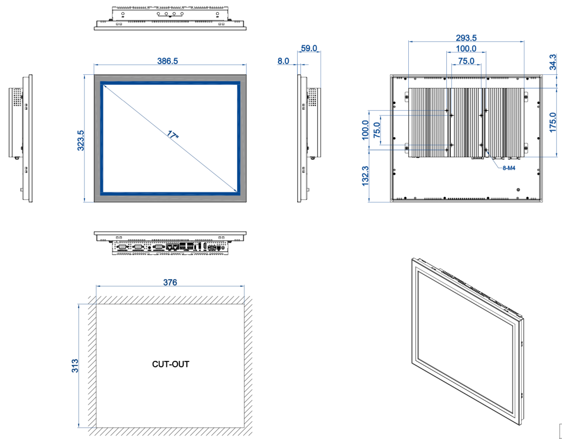
DIMENSIONAL DRAWING:TPC-DRT170D
