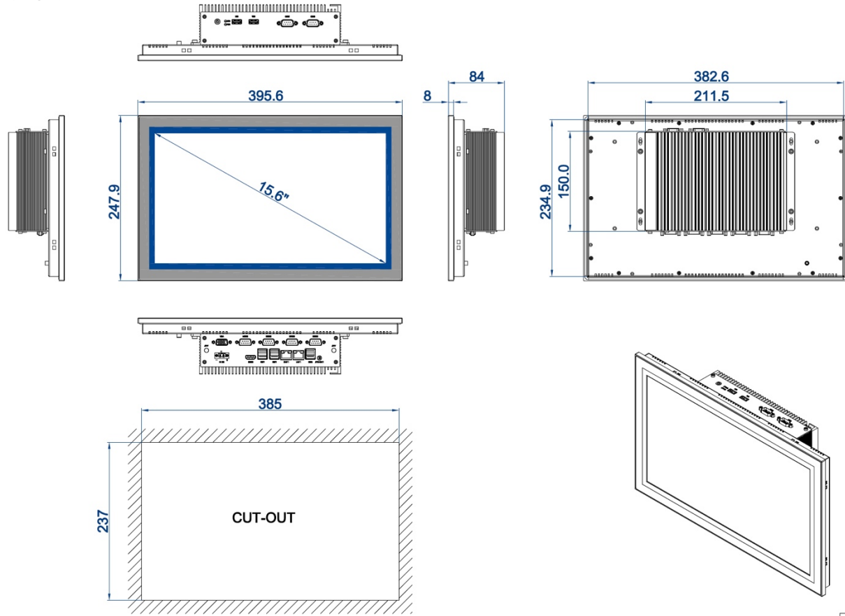
DIMENSIONAL DRAWING:TPC-PR156W
